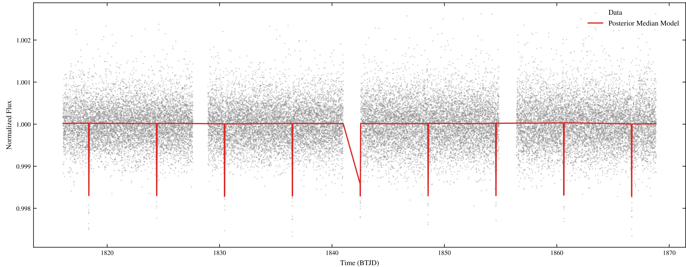
TIC 154840461 | Sectors: 19, 20 | MCMC Posterior Predictive Check
