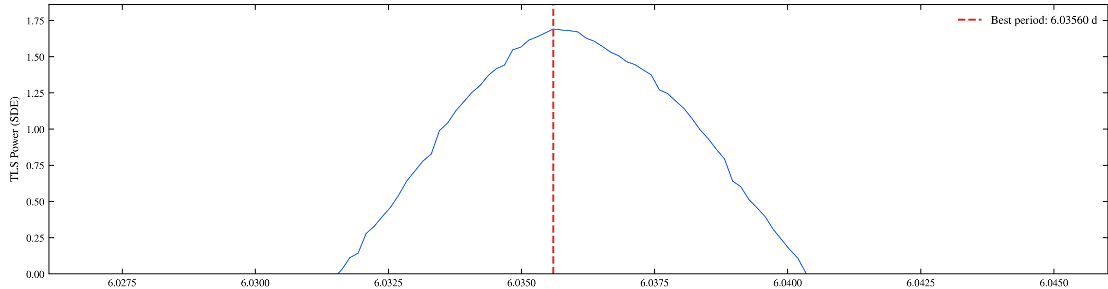
TIC 154840461 | Sectors: 19, 20 | TLS Periodogram (Planet 2 Search) (SDE = 4.96)
