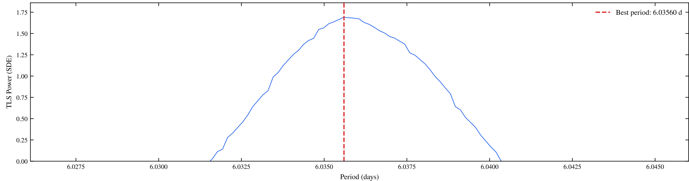
TIC 154840461 | Sectors: 19, 20 | TLS Coarse Periodogram (SDE = 1.69)
