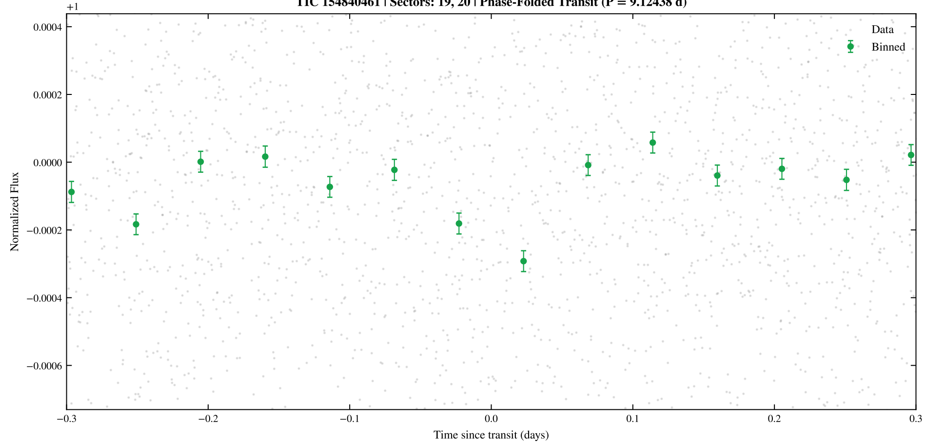
TIC 154840461 | Sectors: 19, 20 | Phase-Folded Transit (P = 9.12438 d)
