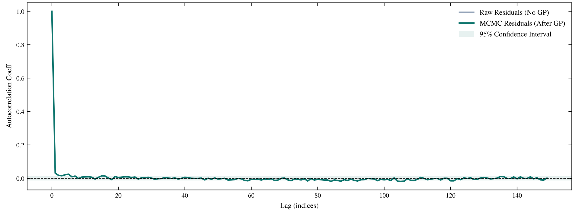
TIC 154840461 | Sectors: 19, 20 | GP Residuals Autocorrelation Function (ACF)
