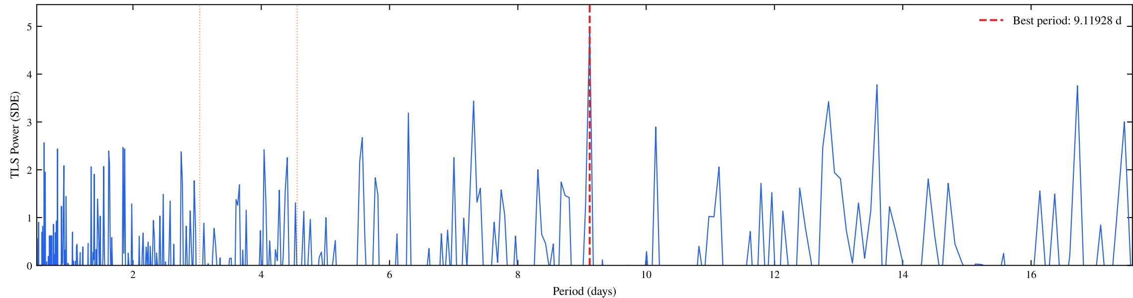
TIC 154840461 | Sectors: 19, 20 | TLS Coarse Periodogram (SDE = 4.96)
