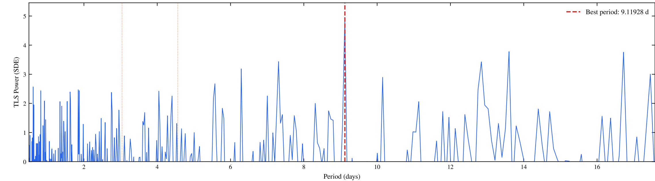
TIC 154840461 | Sectors: 19, 20 | TLS Periodogram (Planet 2 Search) (SDE = 4.96)
