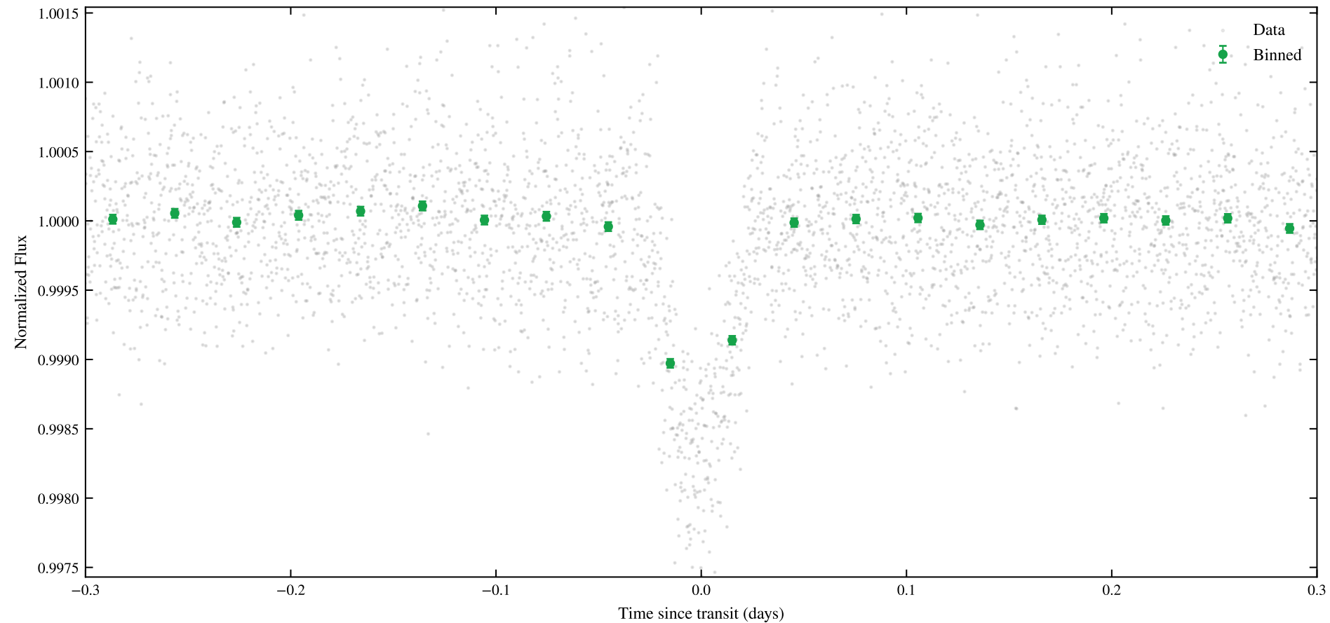
TIC 154840461 | Sectors: 19, 20 | Phase-Folded Transit (P = 6.03560 d)
