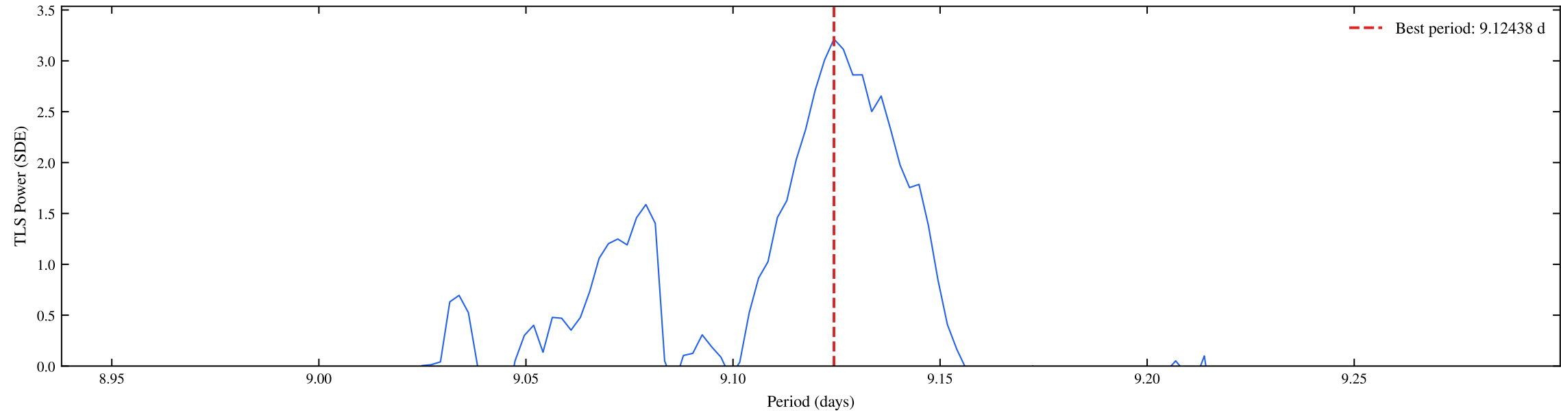
TIC 154840461 | Sectors: 19, 20 | TLS Fine Periodogram (SDE = 3.21)
