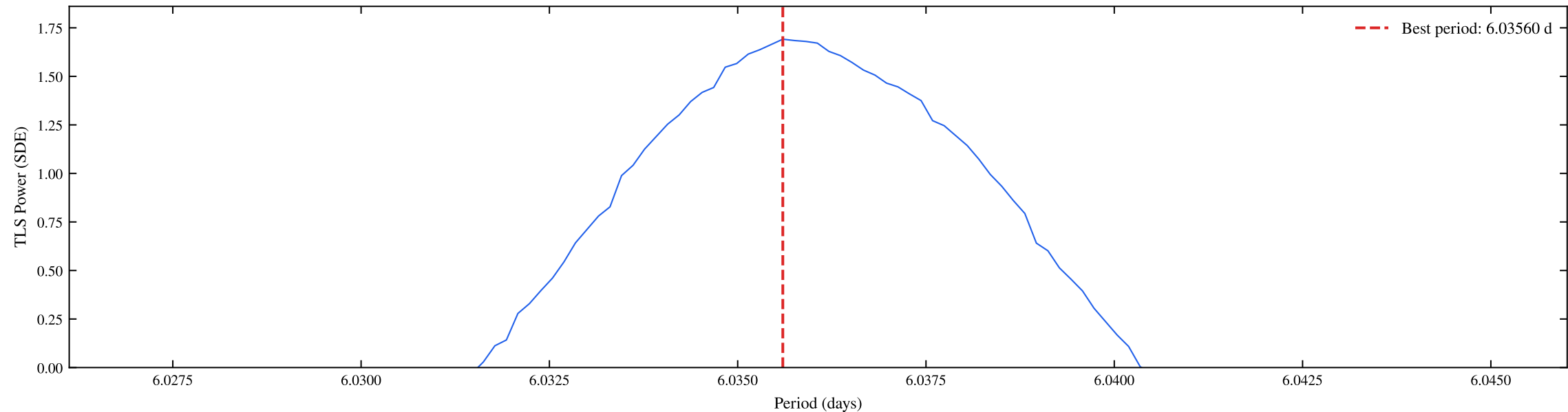
TIC 154840461 | Sectors: 19, 20 | TLS Fine Periodogram (SDE = 1.69)
